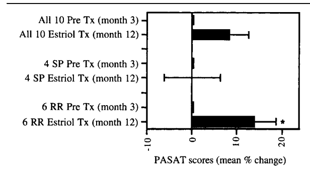
Fig 4. Clinical measures of disease activity. Paced auditory serial addition (PASAT) cognitive testing was performed at study month 3 in the pretreatment m9375(mea3 29(m939375(mea.29(m93
